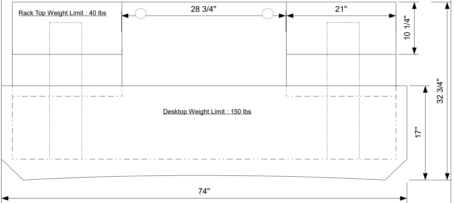
Side View
